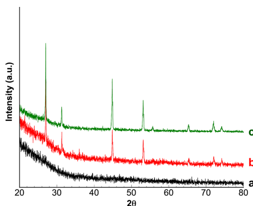
Figure 1. XRD patterns for (a) cross-linked \text{Li}_2\text{S}_3 –PAN after vacuum drying; (b) \text{Li}_2\text{S}_3 –PAN after heat treatment (dehydrogenation and cyclization) at 300^\circ\text{C} ; and (c) \text{Li}_2\text{S} –C after carbonization at 600^\circ\text{C} .
