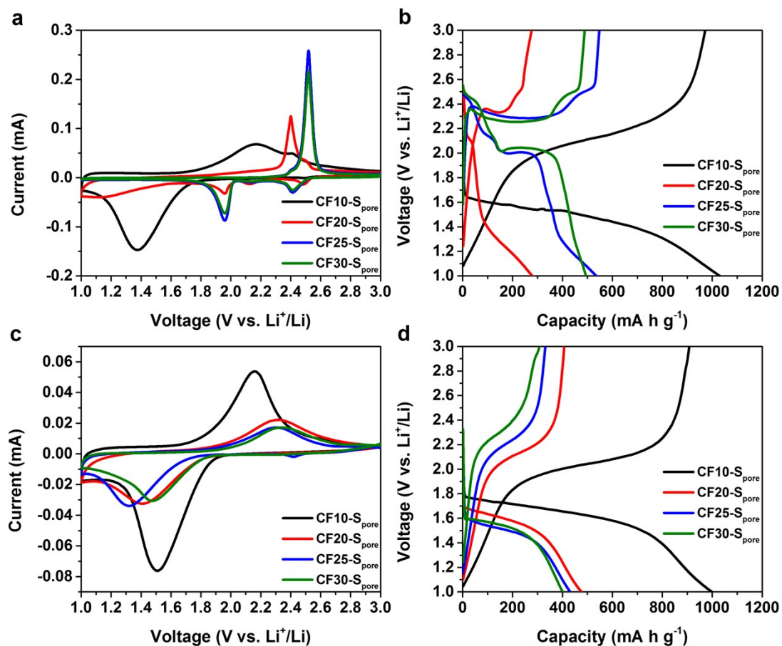
Figure S7. The second CV scans at 0.1 \text{ mV S}^{-1} and the second GCD curves at 160 \text{ mA g}^{-1} of CF10-S pore , CF20-S pore , CF25-S pore , and CF30-S pore in TEGDME electrolyte (a) and (b) respectively, and in EC/DEC electrolyte (c) and (d), respectively.
