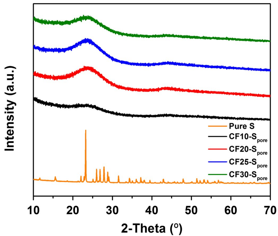
Figure S6. XRD spectra of CF10-S pore , CF20-S pore , CF25-S pore , and CF30-S pore .
