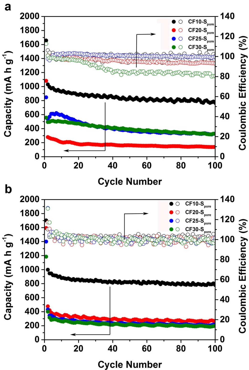
Figure S8. Cycle stability of CF10-S pore , CF20-S pore , CF25-S pore , and CF30-S pore at 160 mA g -1 in (a) TEGDME electrolyte and (b) EC/DEC electrolyte.
