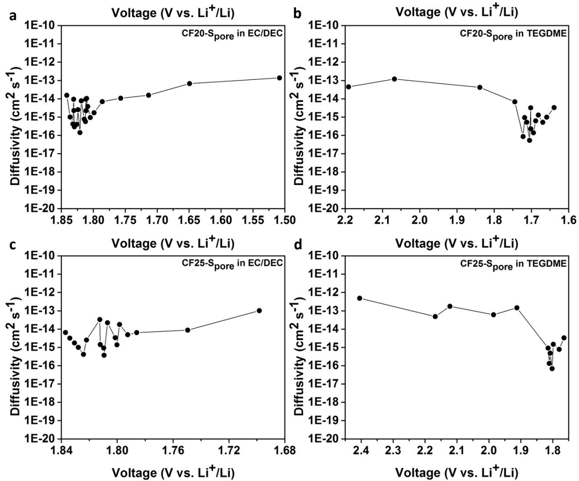
Figure S10. Li diffusivity calculated from the GITT data of CF20-S pore in (a) EC/DEC and (b) TEGDME electrolytes; CF25-S pore in (c) EC/DEC and (d) TEGDME electrolytes.
