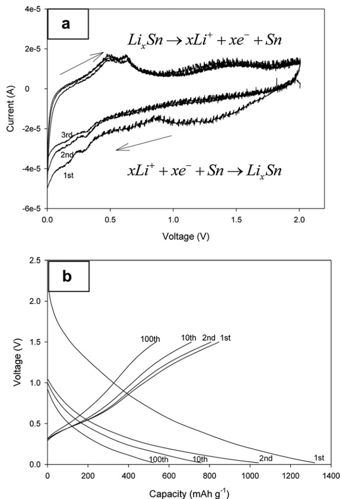
Fig. 3. (a) Cyclic voltammograms at 0.2 \text{ mV s}^{-1} and (b) charge-discharge curves at 1 \text{ A g}^{-1} current of Sn/Ni/TMV1cys anode.
